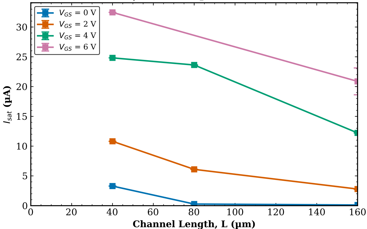
TFT2 Combined (Tr. 1 & 2) I_{sat} vs L | W = 500 \mu\text{m} (mean \pm std)
